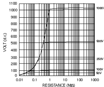
Typical Terminal Voltage Characteristics:
